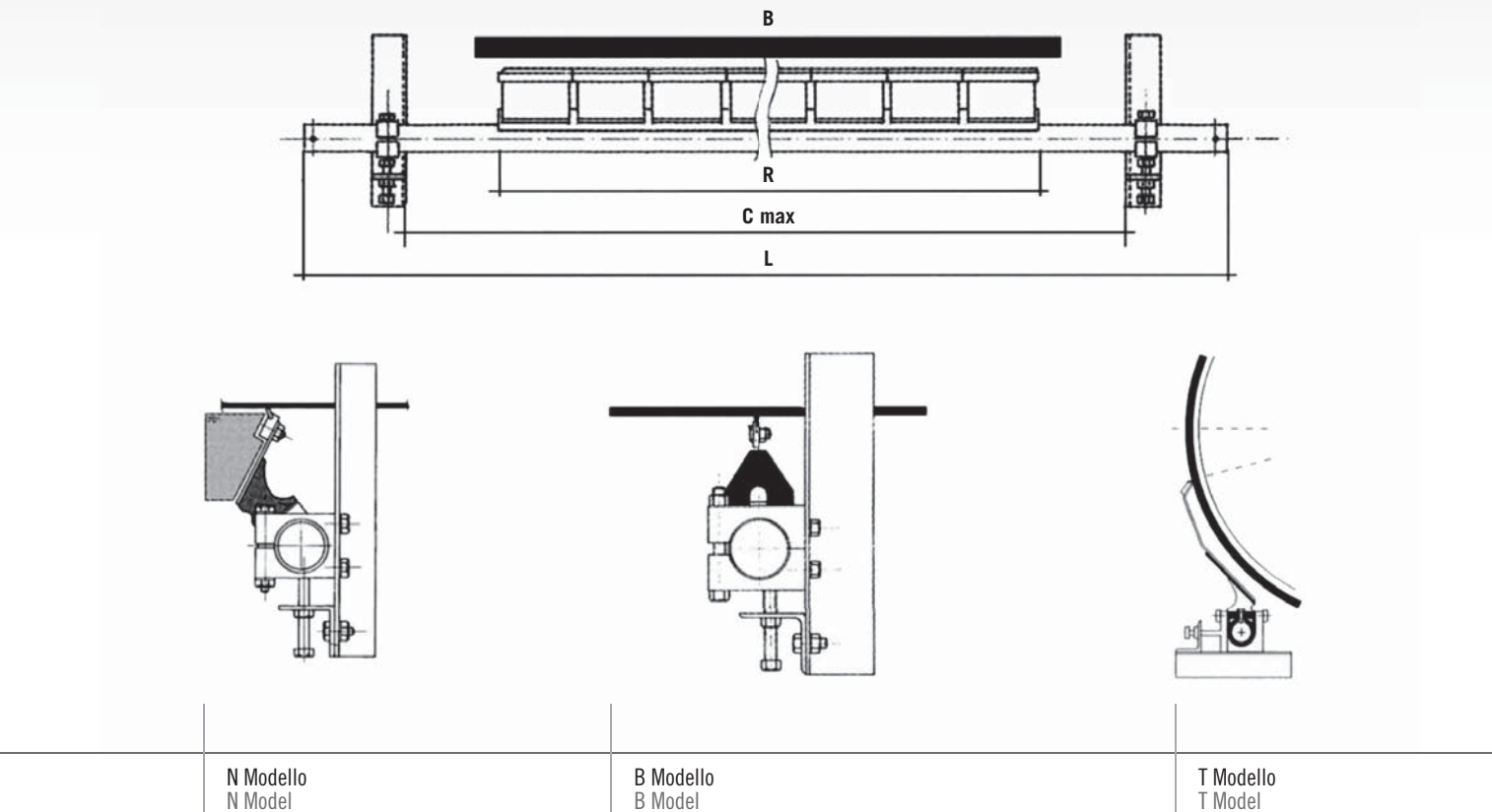
DIMENSIONI STANDARD STANDARD DIMENSIONS
