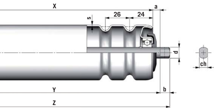
RULLO GAMMA 2G GAMMA ROLLER 2G
