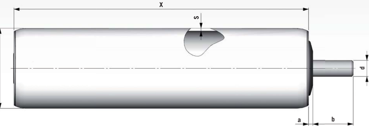
RULLO A SBALZO GAMMA - DELTA GAMMA - DELTA CANTILEVER ROLLER
