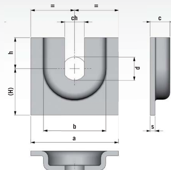
Supporto 200.1 - 2 - 3 Support 200.1 - 2 - 3
