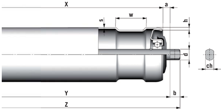
RULLO GAMMA GOLA PIANA GAMMA ROLLERS FLAT GROOVES
